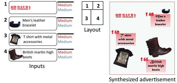
Figure 16: Advertisement example synthesized by our approach.
