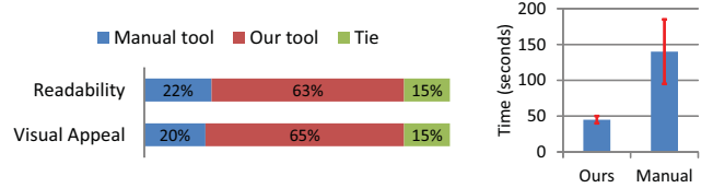
Figure 12: Results from pairwise comparisons of compositions by our tool and the manual tool. Left: each number in the bar shows the percentage of votes from the evaluators. The evaluators preference for the compositions by our approach is statistically significant ( p < 0.05 , chi-squared test, 2 dof). Right: average time of generating one composition by our tool and manual tool.
